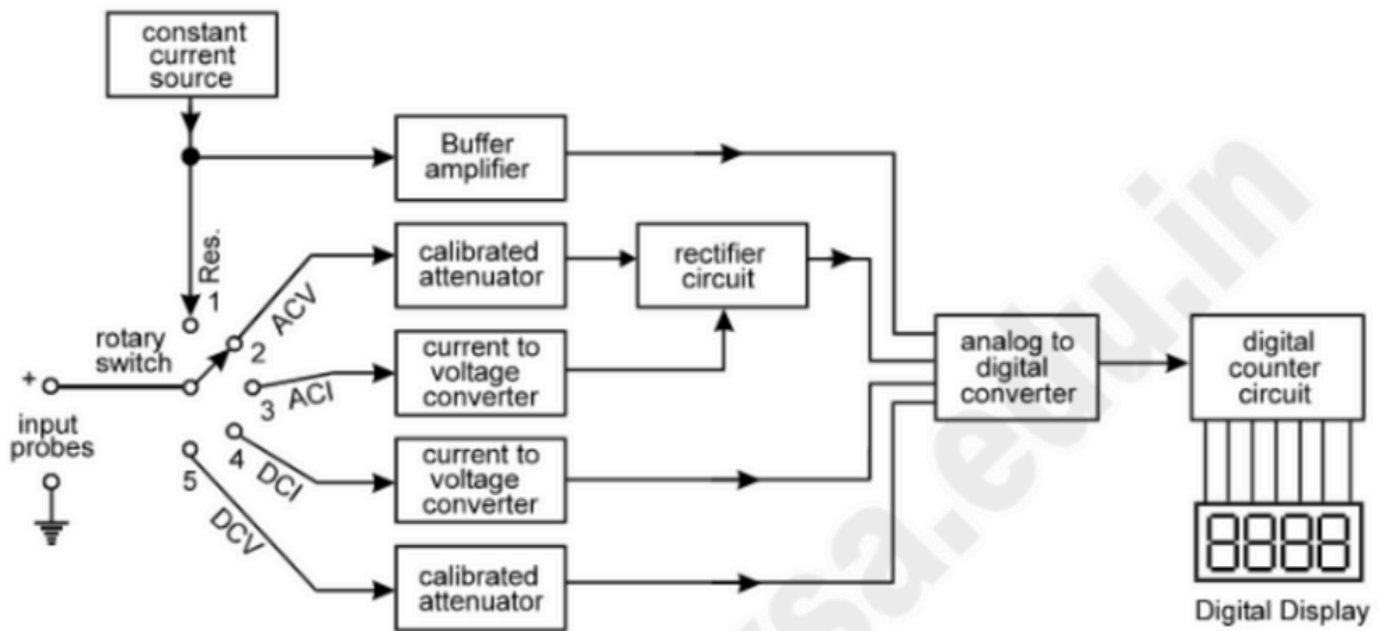
Block diagram of basic digital multimeter
